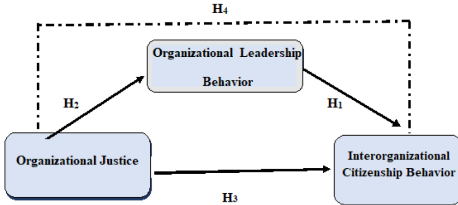
Figure 1. Research Model
